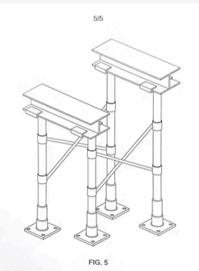
I Beam Tower Stand With Cross Bracing
