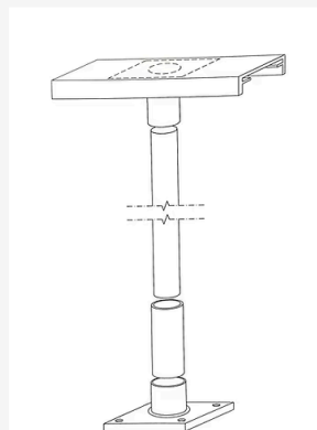
Single Leg Pipe Stand
